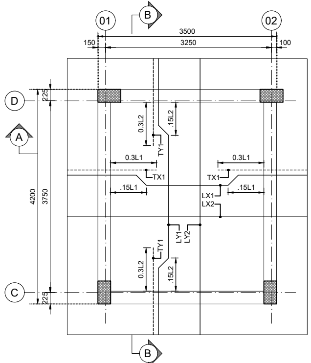
MUMMTY SLAB REINFORCEMENT DETAILS
